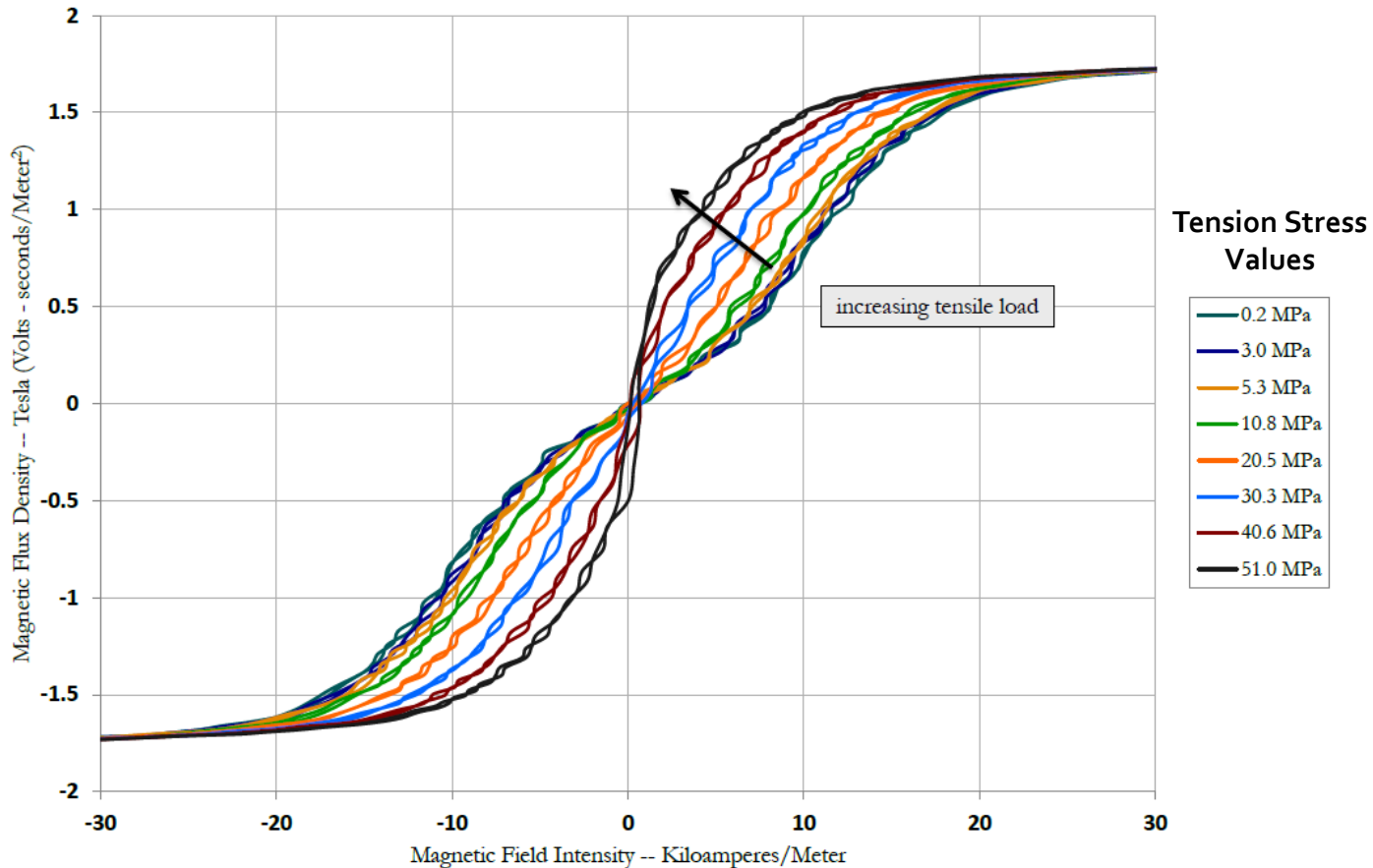
Galfenol Stress Annealed BH - Tested under tension Magnetic Flux vs. Magnetic Field
