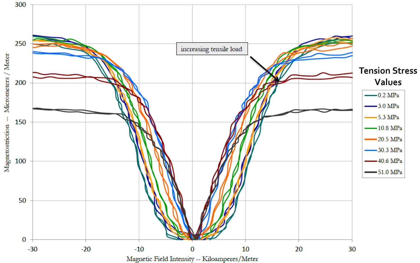
Galfenol Stress Annealed SH - Tested under tension Magnetostriction vs. Magnetic Field
